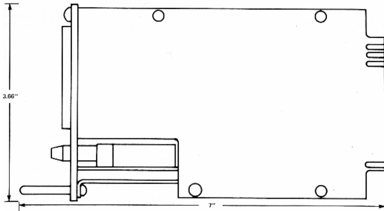
MECHANICAL LAYOUT
