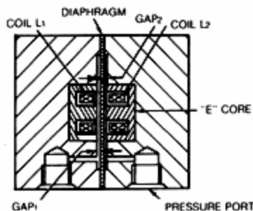
FIGURE 1. Typical Transducer Cross-Section
