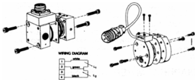
FIGURE 4. Typical Transducer Assemblies
