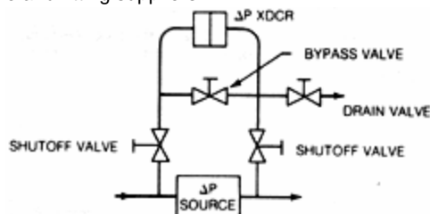
FIGURE 3. Typical Valve Arrangement for DP Use
