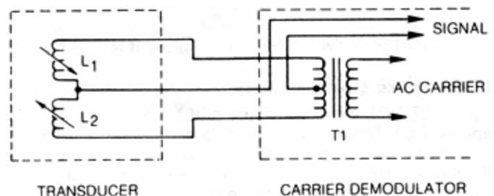
FIGURE 2. Transducer Bridge Circuit
